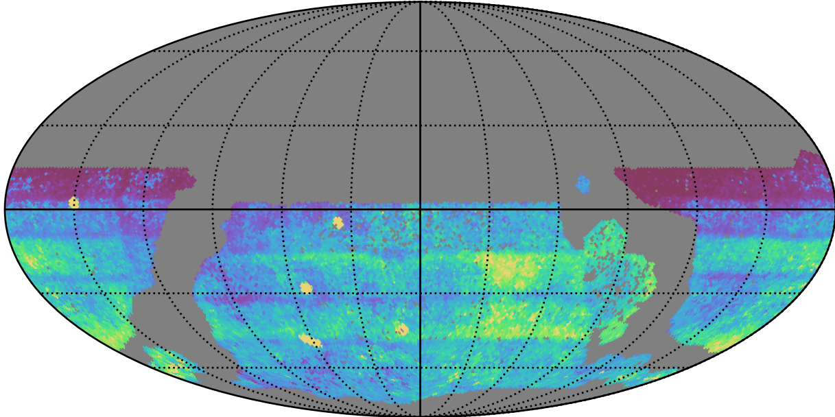
too_elab_r64_d3_giz_v3.4_10yrs WFD all bands: 75th Percentile Intranight Timespan
