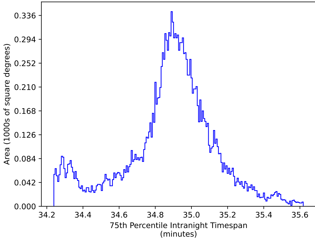
too_elab_r64_d3_giz_v3.4_10yrs WFD: 75th Percentile Intranight Timespan
