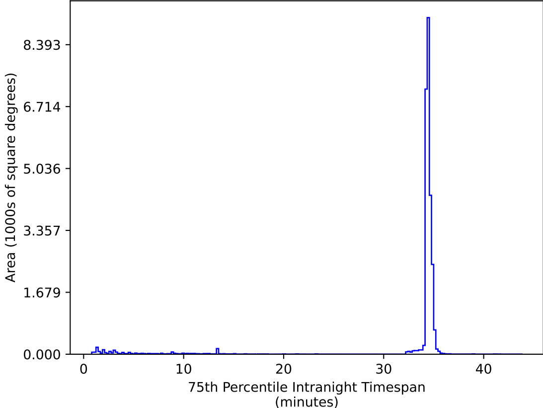
too_elab_r64_d3_giz_v3.4_10yrs All sky zy bands: 75th Percentile Intranight Timespan
