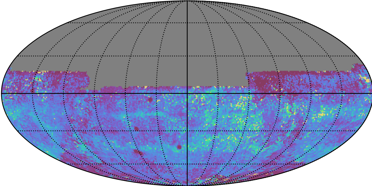
too_elab_r64_d3_giz_v3.4_10yrs All sky y band: 75th Percentile Intranight Timespan
