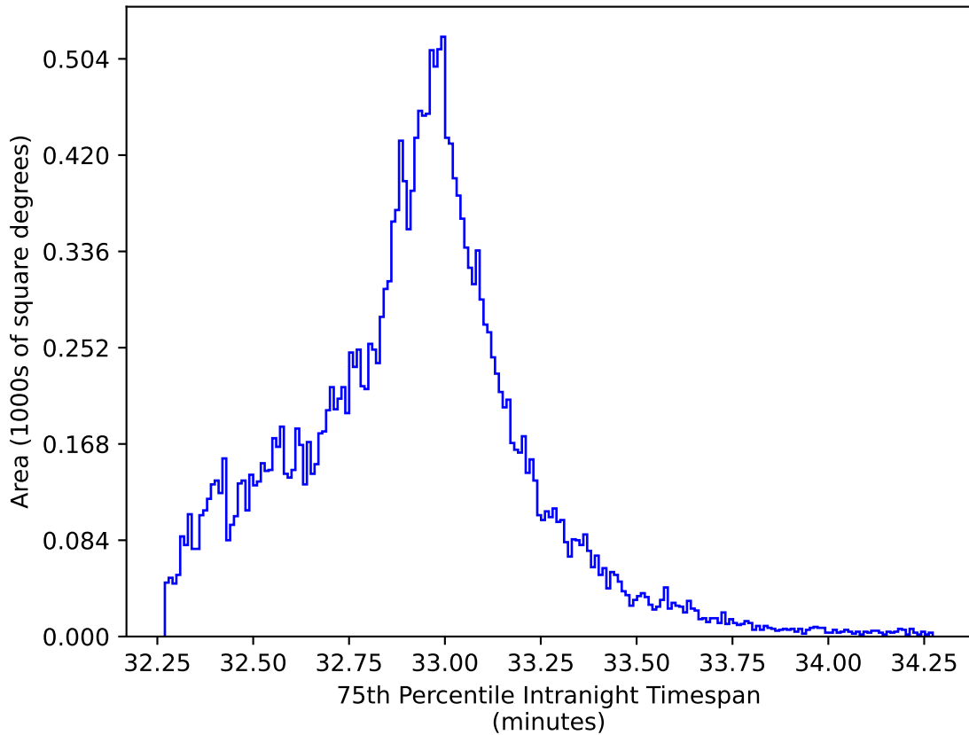
too_elab_r64_d3_giz_v3.4_10yrs All sky y band: 75th Percentile Intranight Timespan
