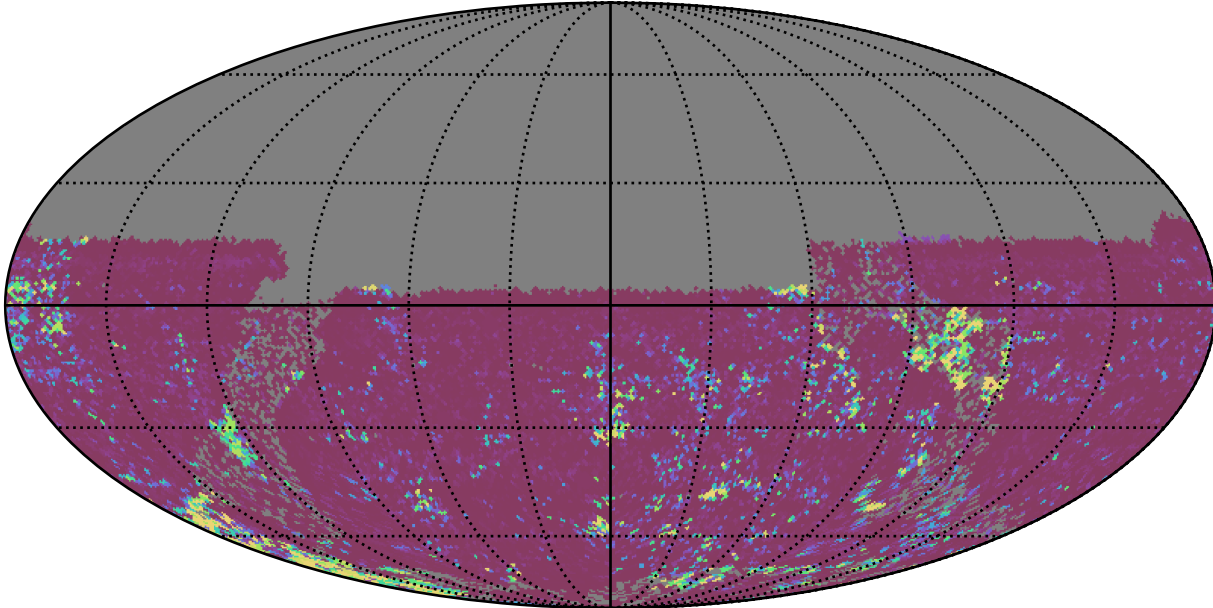
too_elab_r64_d3_giz_v3.4_10yrs All sky u band: 75th Percentile Intranight Timespan
