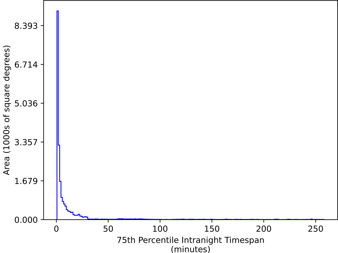
too_elab_r64_d3_giz_v3.4_10yrs All sky u band: 75th Percentile Intranight Timespan
