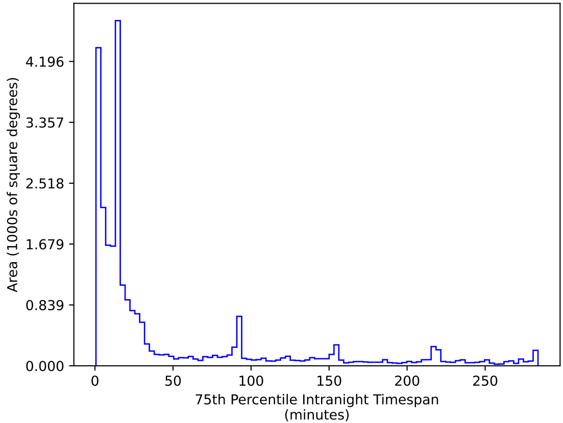
too_elab_r64_d3_giz_v3.4_10yrs All sky r band: 75th Percentile Intranight Timespan
