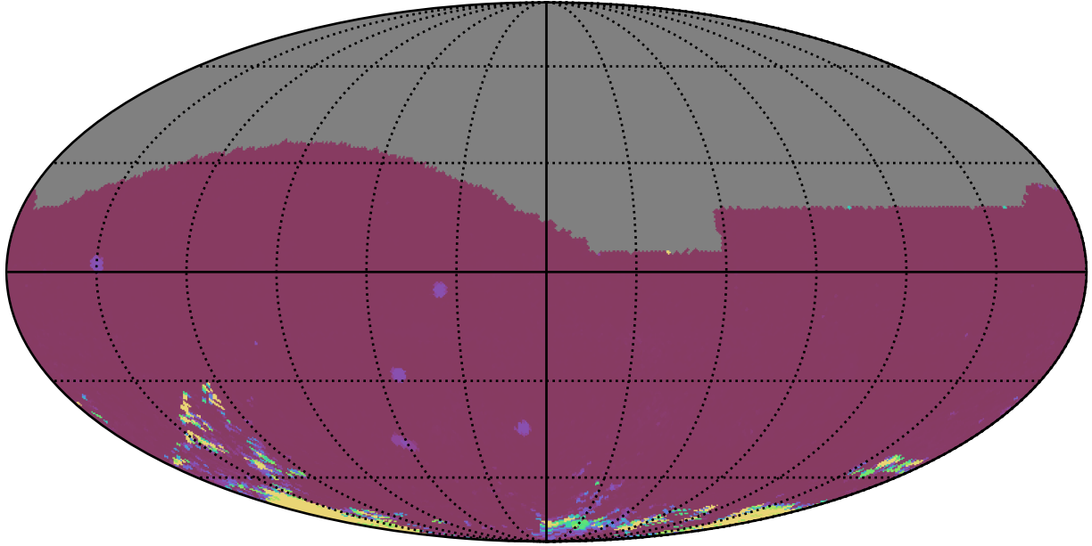
too_elab_r64_d3_giz_v3.4_10yrs All sky iz bands: 75th Percentile Intranight Timespan
