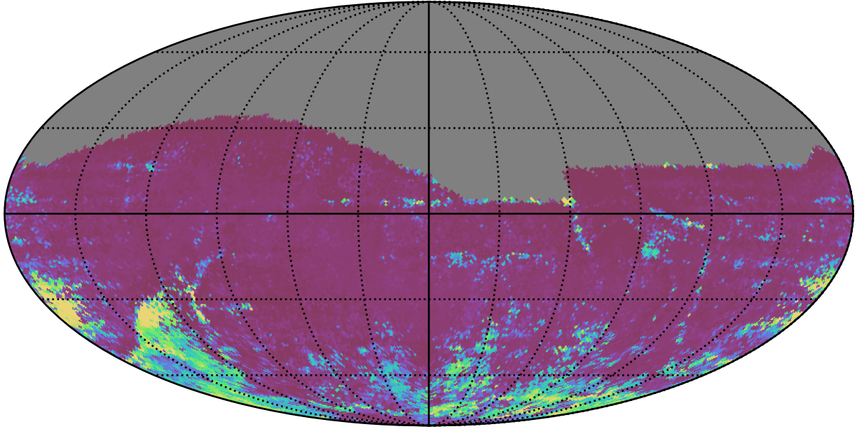
too_elab_r64_d3_giz_v3.4_10yrs All sky i band: 75th Percentile Intranight Timespan
