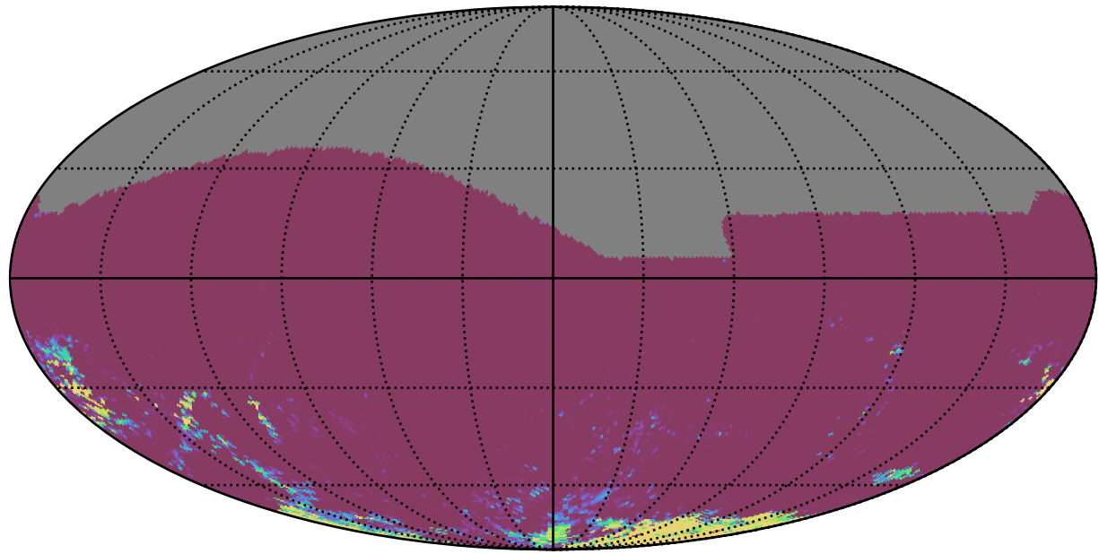
too_elab_r64_d3_giz_v3.4_10yrs All sky gr bands: 75th Percentile Intranight Timespan
