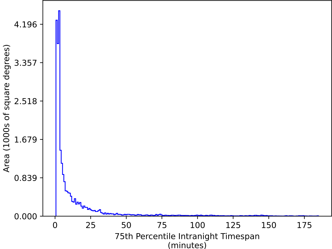
too_elab_r64_d3_giz_v3.4_10yrs All sky g band: 75th Percentile Intranight Timespan
