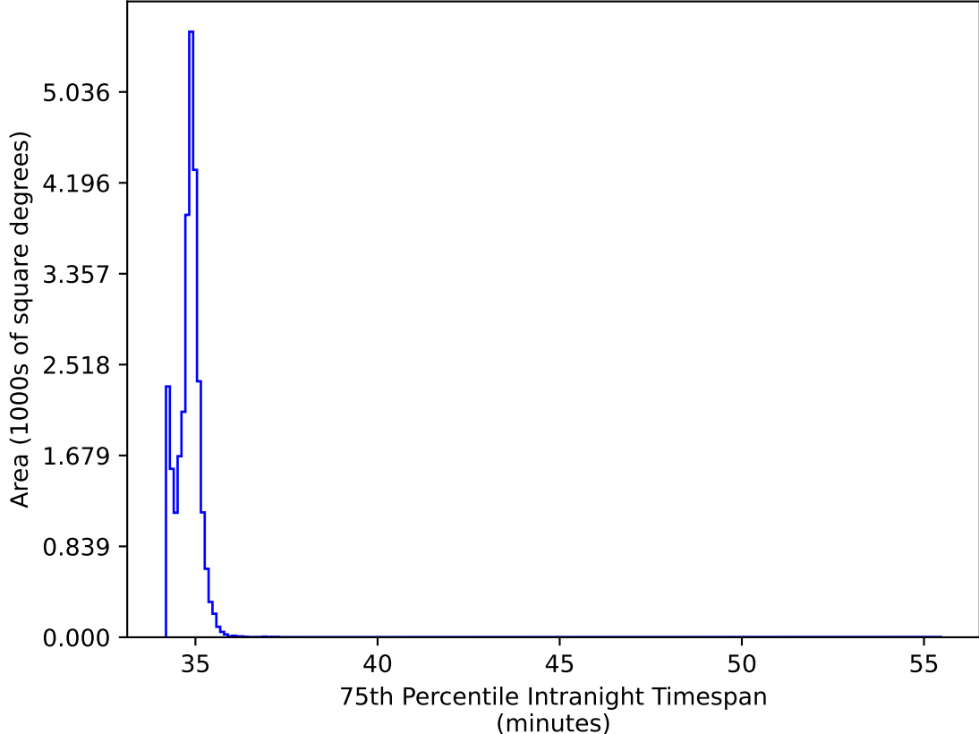
too_elab_r64_d3_giz_v3.4_10yrs All sky all bands: 75th Percentile Intranight Timespan
