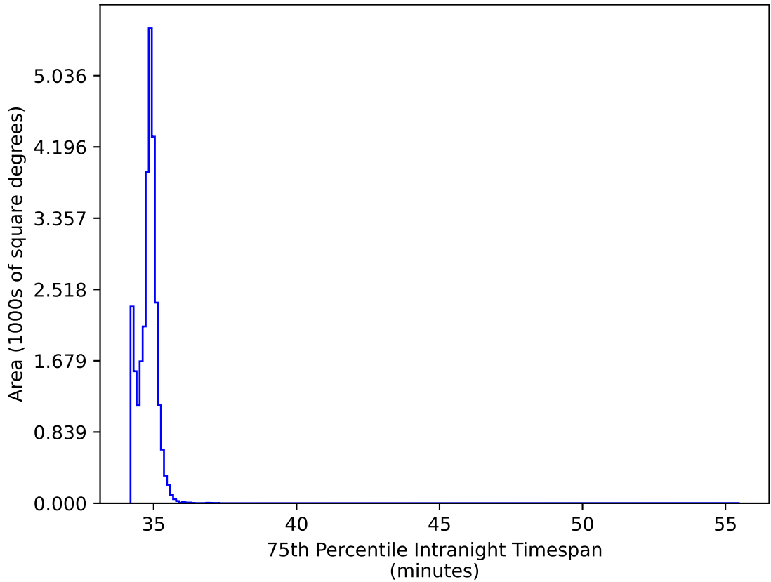
too_elab_r64_d3_giz_v3.4_10yrs All sky: 75th Percentile Intranight Timespan
