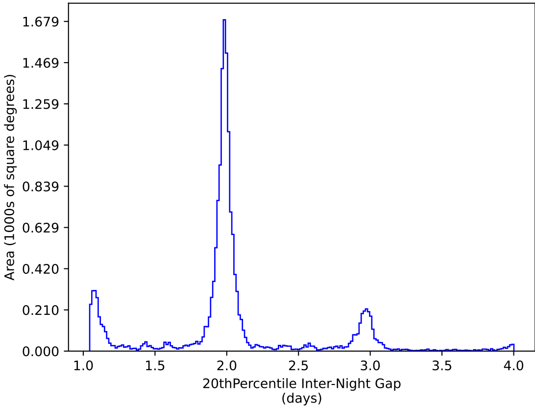
too_elab_r64_d3_giz_v3.4_10yrs WFD y band: 20thPercentile Inter-Night Gap
