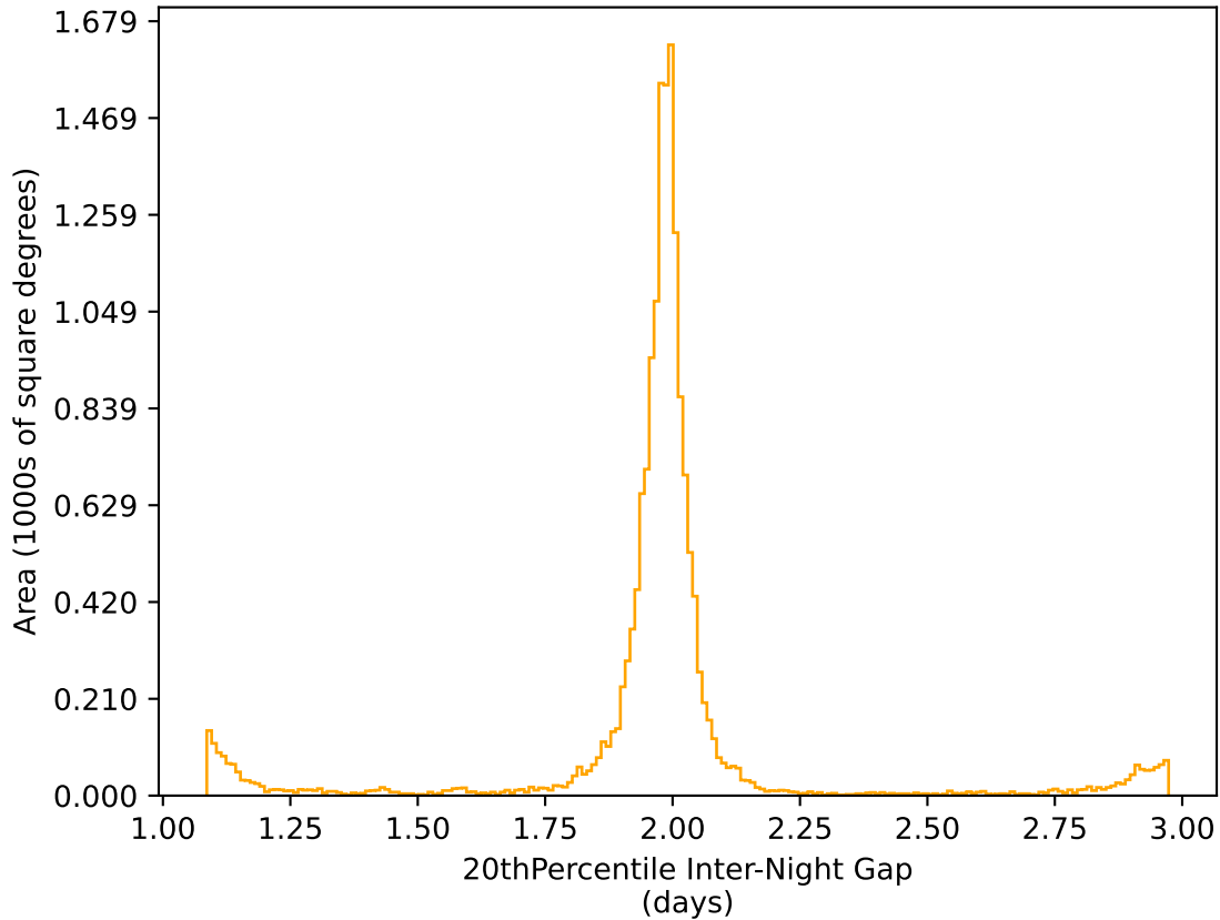
too_elab_r64_d3_giz_v3.4_10yrs WFD r band: 20thPercentile Inter-Night Gap
