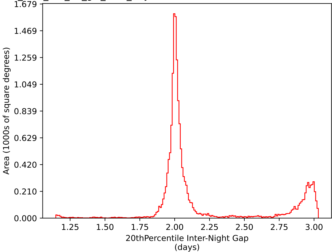
too_elab_r64_d3_giz_v3.4_10yrs WFD i band: 20thPercentile Inter-Night Gap
