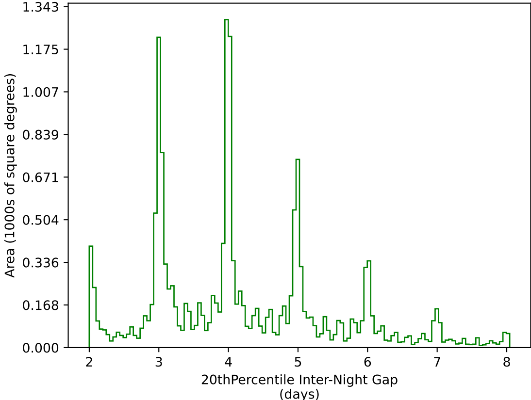
too_elab_r64_d3_giz_v3.4_10yrs WFD g band: 20thPercentile Inter-Night Gap
