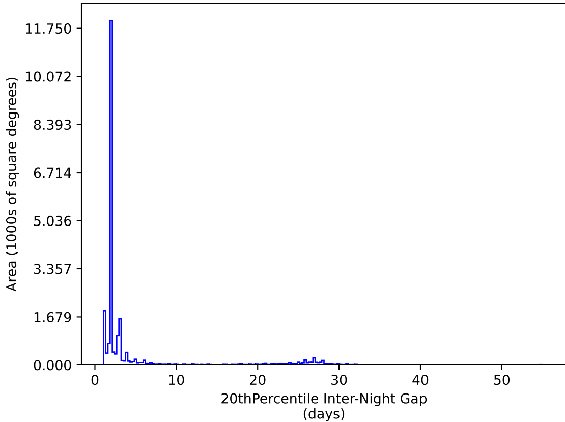
too_elab_r64_d3_giz_v3.4_10yrs All sky y band: 20thPercentile Inter-Night Gap
