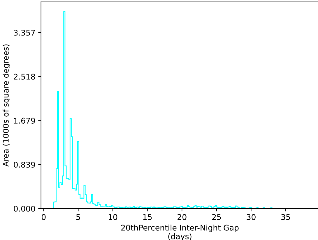
too_elab_r64_d3_giz_v3.4_10yrs All sky u band: 20thPercentile Inter-Night Gap
