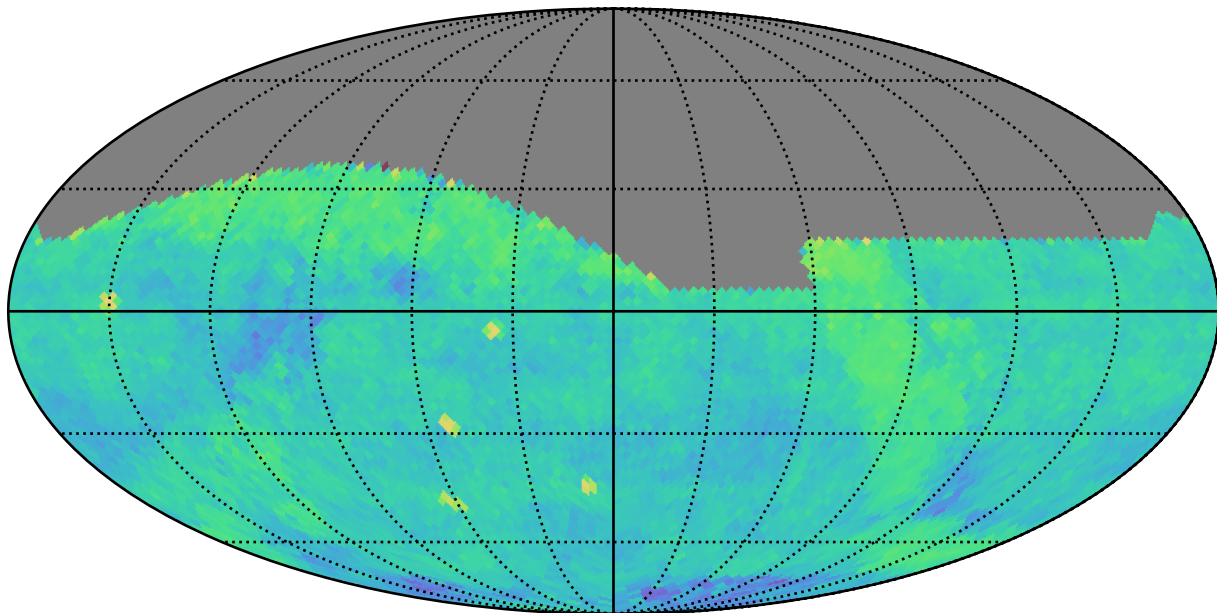
too_elab_r64_d3_giz_v3.4_10yrs (g or r or i): PairFraction
