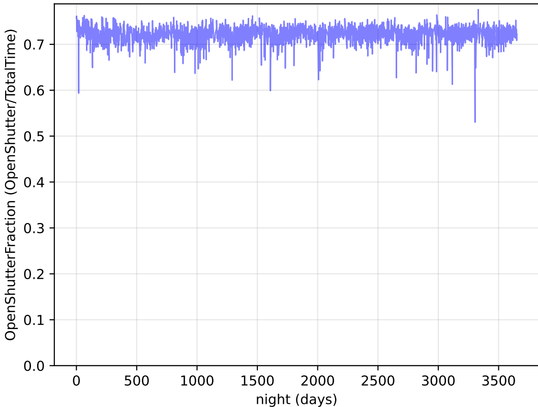
too_elab_r64_d3_giz_v3.4_10yrs : OpenShutterFraction
