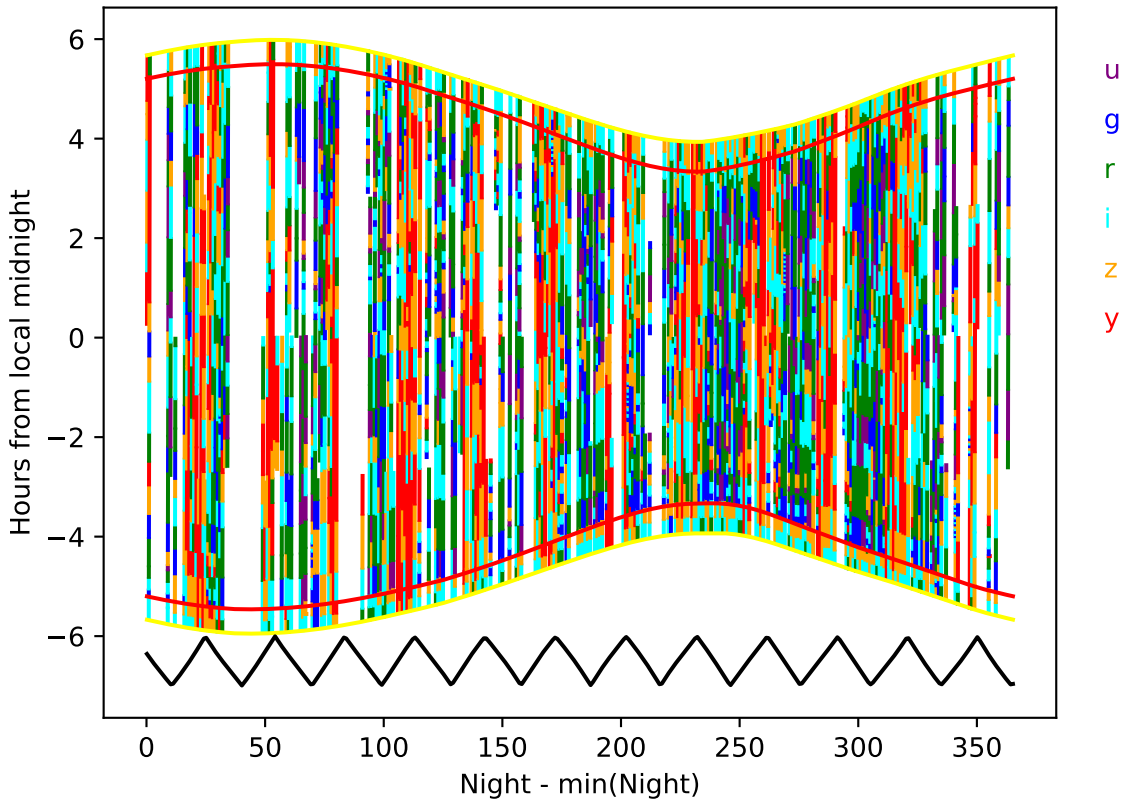
too_elab_r64_d3_giz_v3.4_10yrs year 4-5: Hourglass
