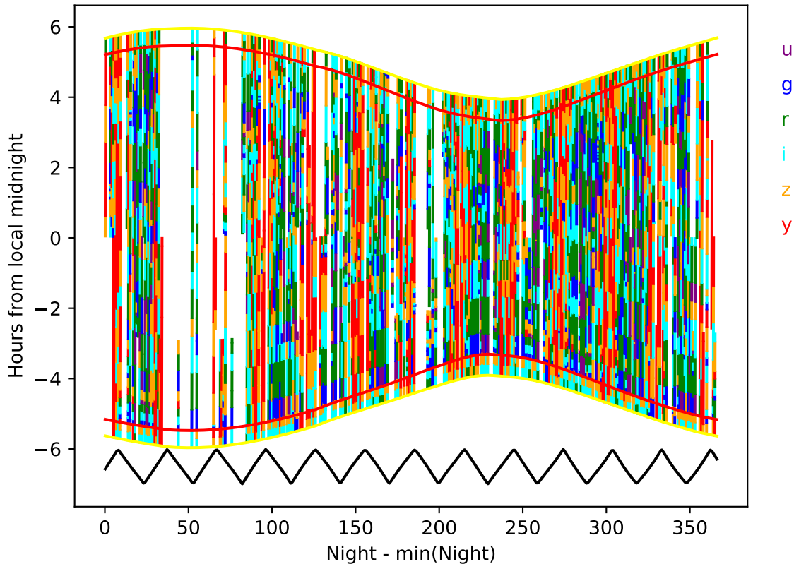
too_elab_r64_d3_giz_v3.4_10yrs year 3-4: Hourglass
