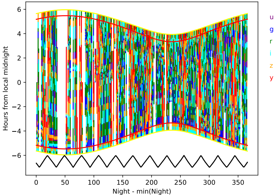
too_elab_r64_d3_giz_v3.4_10yrs year 2-3: Hourglass
