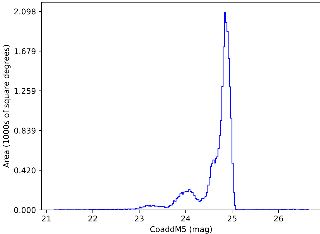
too_elab_r64_d3_giz_v3.4_10yrs y: CoaddM5
