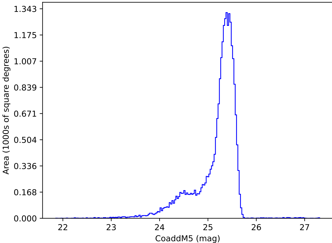
too_elab_r64_d3_giz_v3.4_10yrs u: CoaddM5
