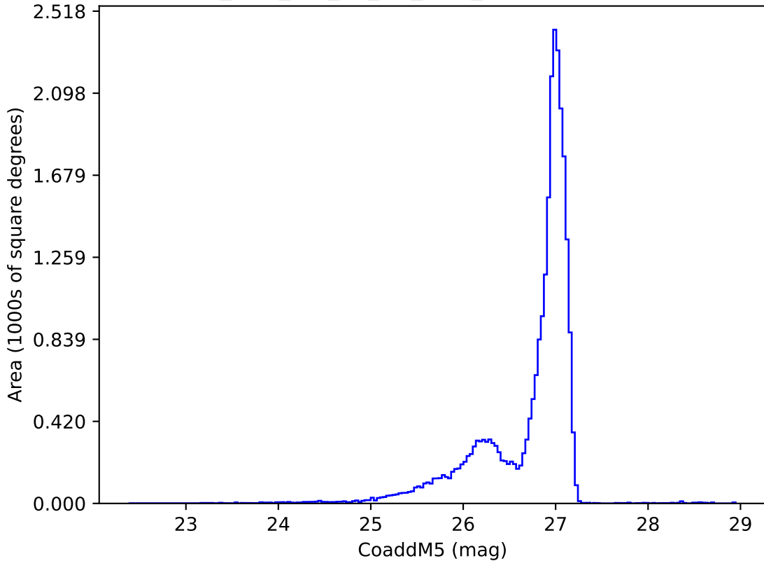
too_elab_r64_d3_giz_v3.4_10yrs r: CoaddM5
