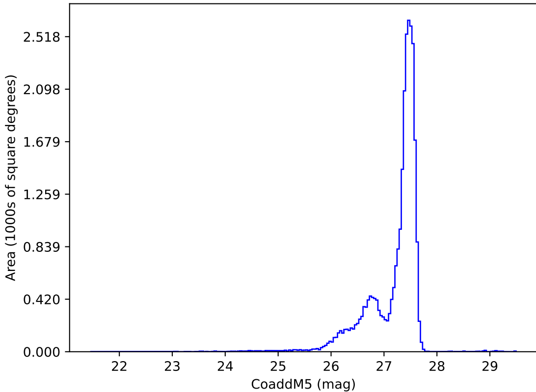
too_elab_r64_d3_giz_v3.4_10yrs : CoaddM5
