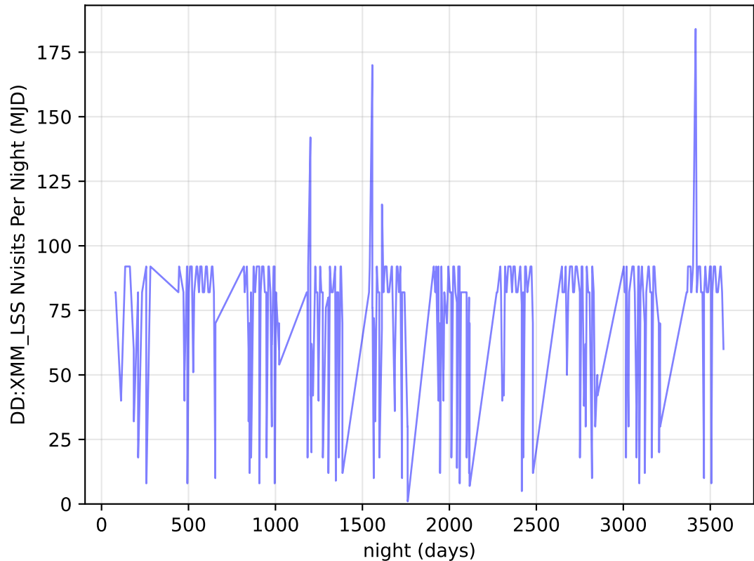
too_elab_r64_d3_giz_v3.4_10yrs all bands: DD:XMM_LSS Nvisits Per Night
