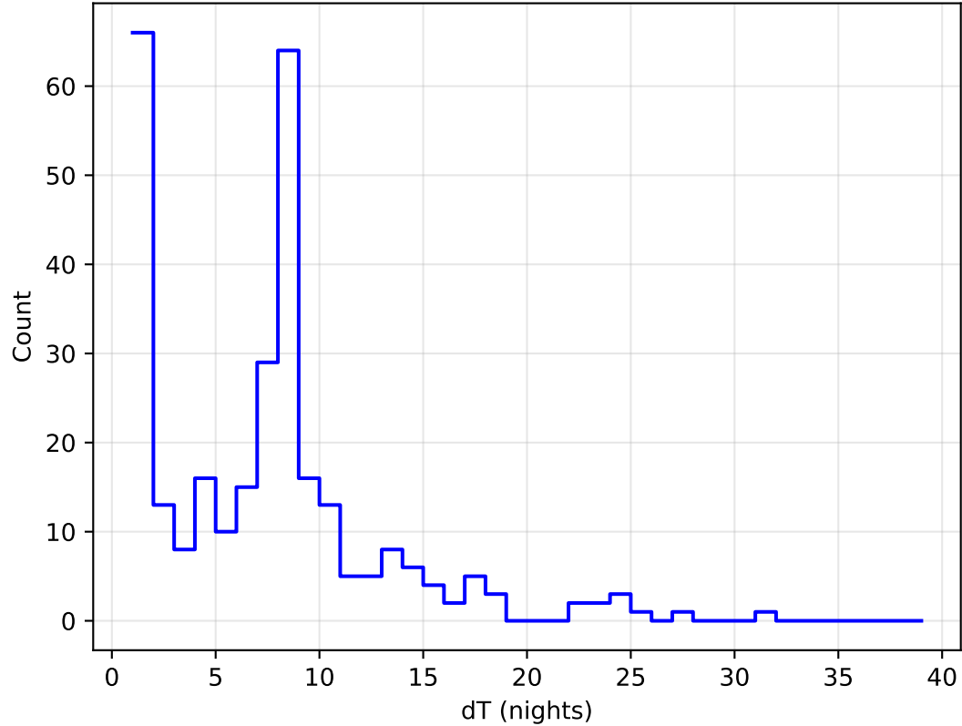
too_elab_r64_d3_giz_v3.4_10yrs all bands: DD:XMM_LSS Delta Nights Histogram
