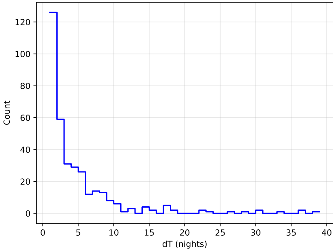
too_elab_r64_d3_giz_v3.4_10yrs all bands: DD:WFD Delta Nights Histogram
