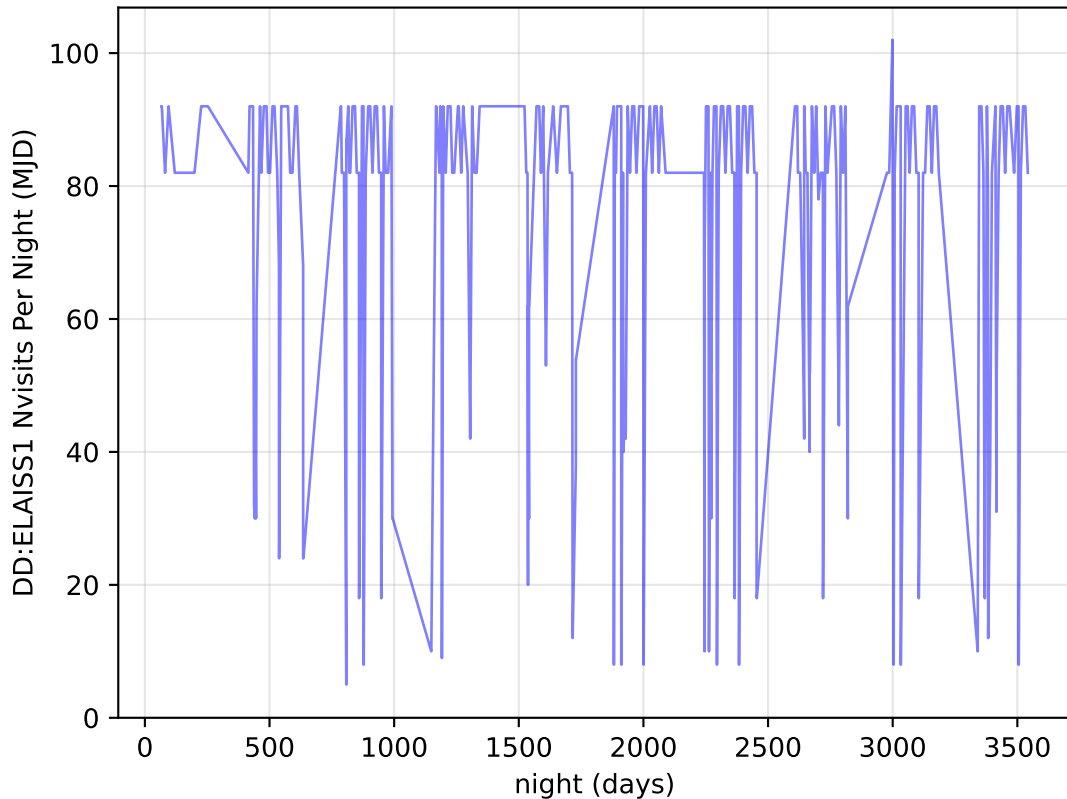
too_elab_r64_d3_giz_v3.4_10yrs all bands: DD:ELAISS1 Nvisits Per Night
