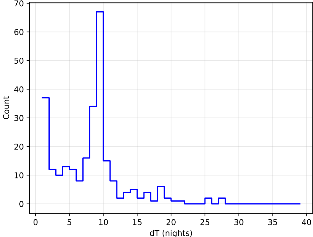
too_elab_r64_d3_giz_v3.4_10yrs all bands: DD:ELAISS1 Delta Nights Histogram
