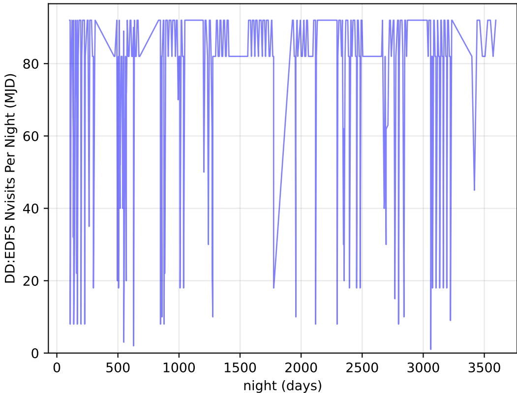
too_elab_r64_d3_giz_v3.4_10yrs all bands: DD:EDFS Nvisits Per Night
