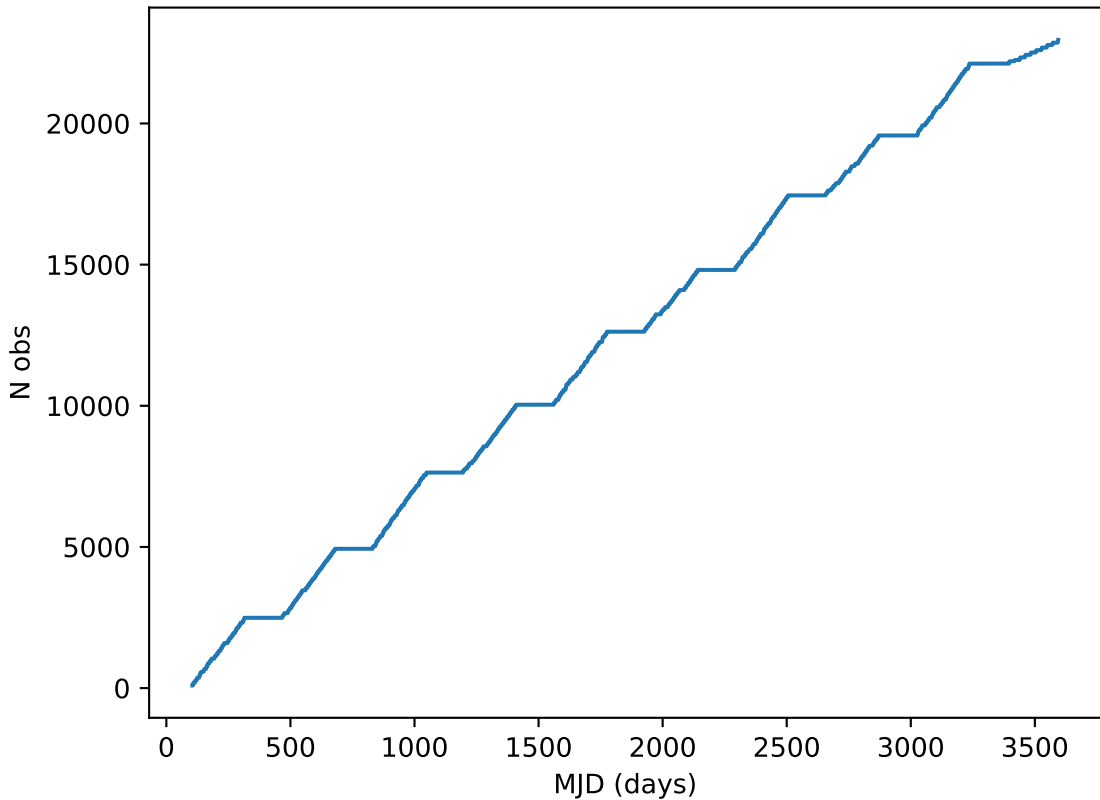
too_elab_r64_d3_giz_v3.4_10yrs all bands: DD:EDFS Cumulative NVisits
