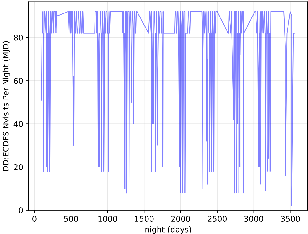
too_elab_r64_d3_giz_v3.4_10yrs all bands: DD:ECDFS Nvisits Per Night
