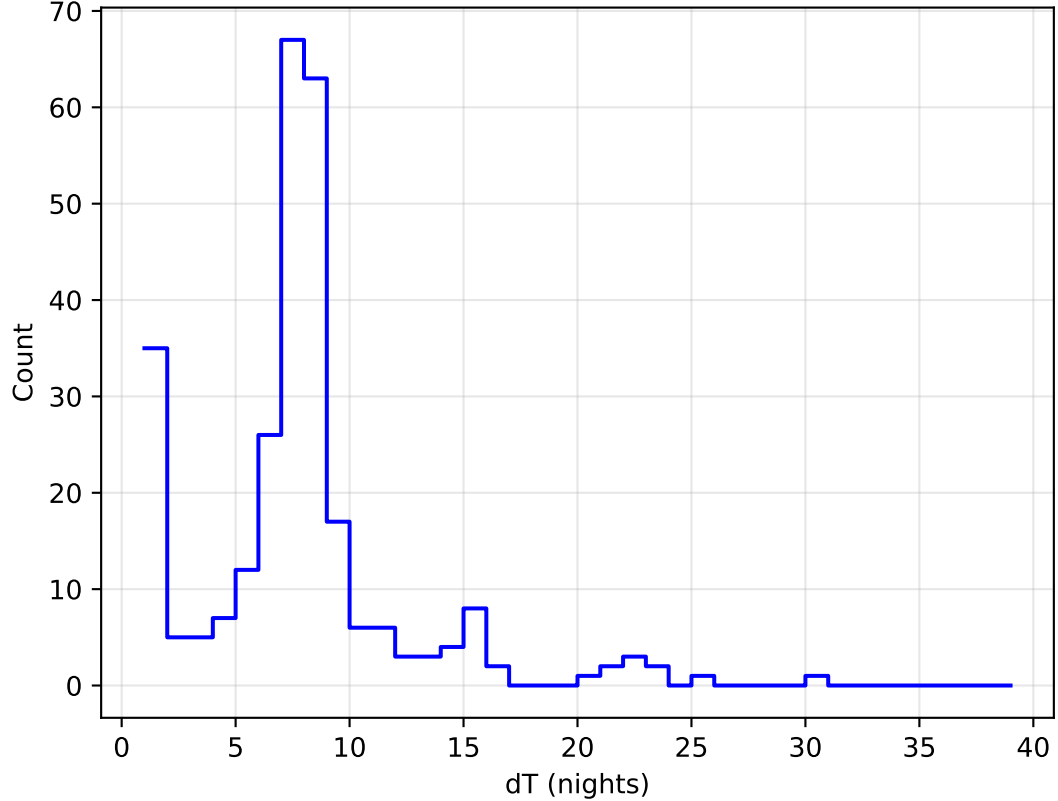
too_elab_r64_d3_giz_v3.4_10yrs all bands: DD:ECDFS Delta Nights Histogram
