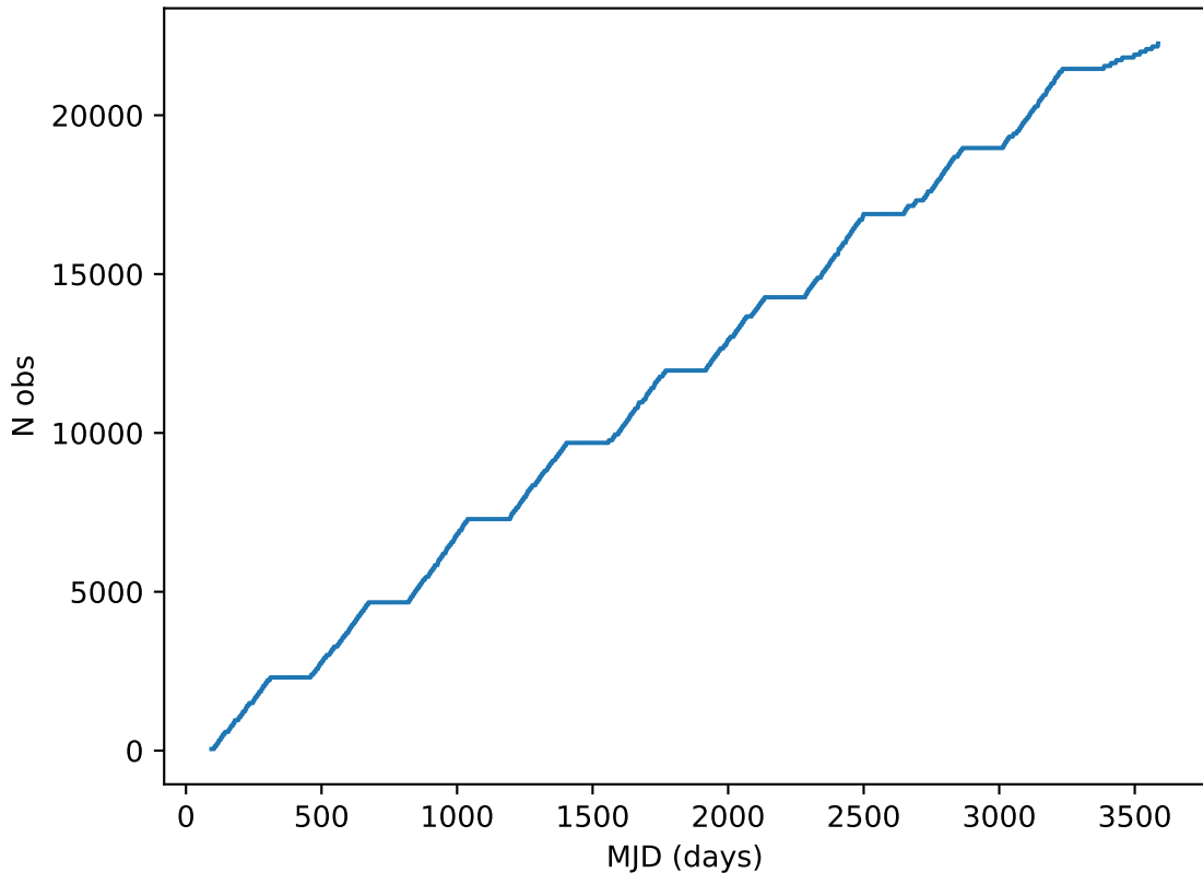
too_elab_r64_d3_giz_v3.4_10yrs all bands: DD:ECDFS Cumulative NVisits
