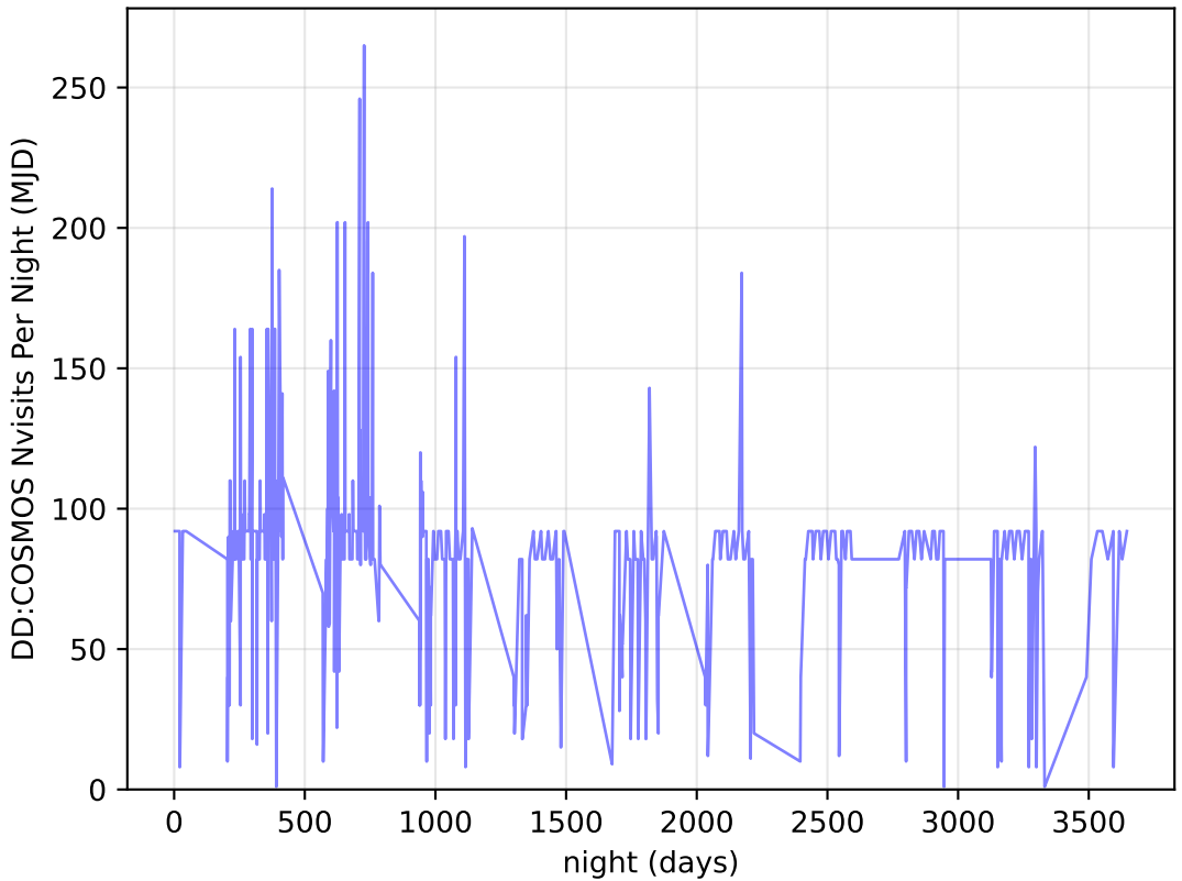
too_elab_r64_d3_giz_v3.4_10yrs all bands: DD: COSMOS Nvisits Per Night
