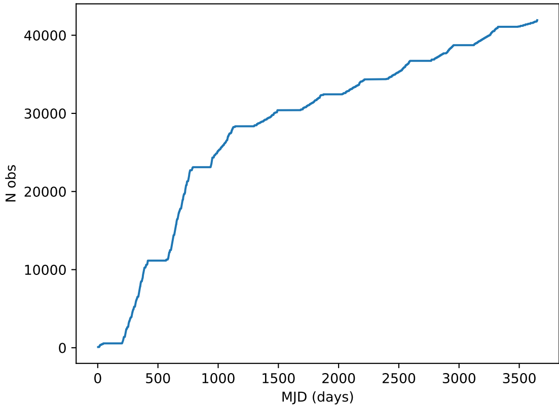
too_elab_r64_d3_giz_v3.4_10yrs all bands: DD:COSMOS Cumulative NVisits
