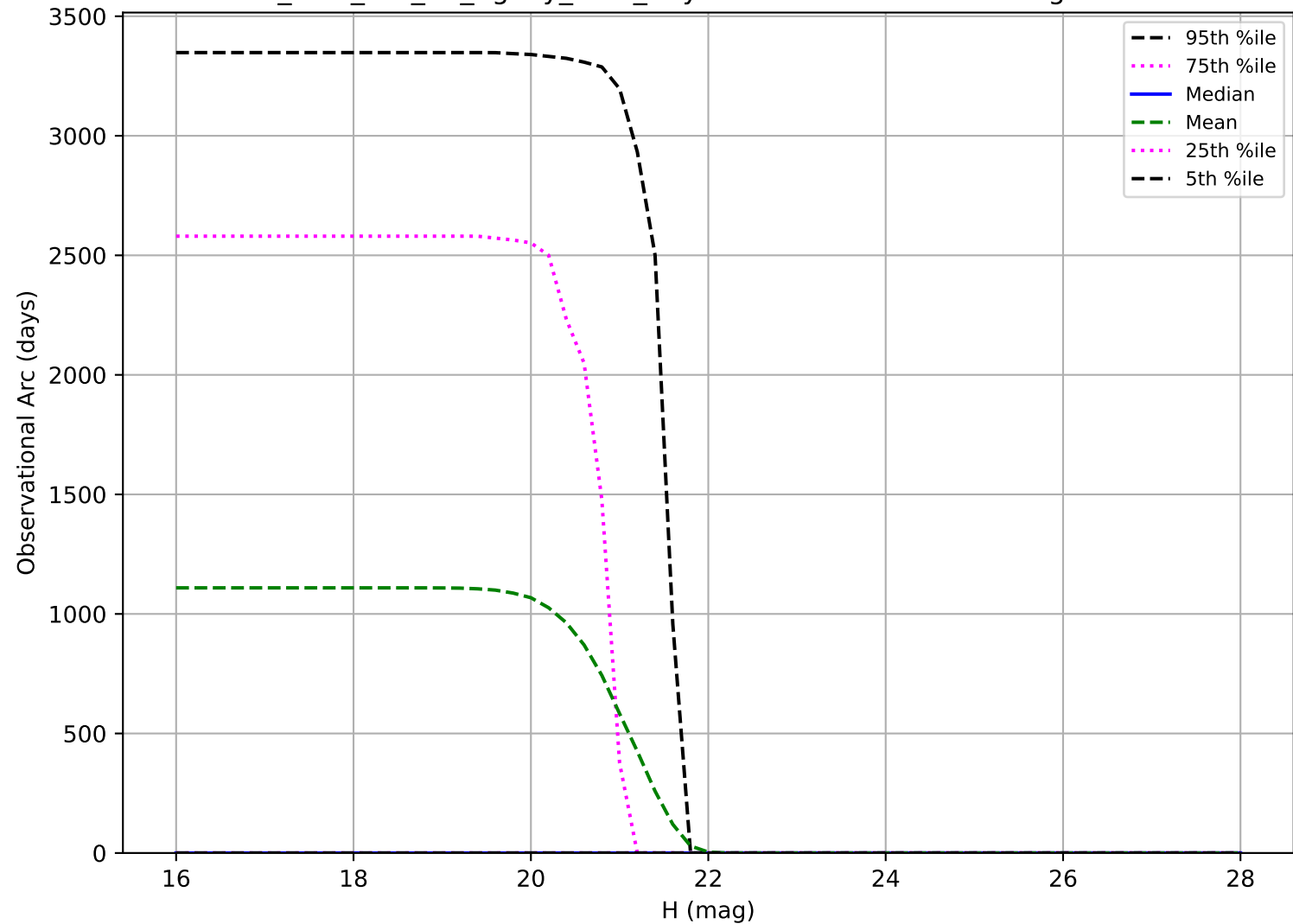
too_elab_r64_d2_ugrizy_v3.4_10yrs: Observational Arc Length Vatra
