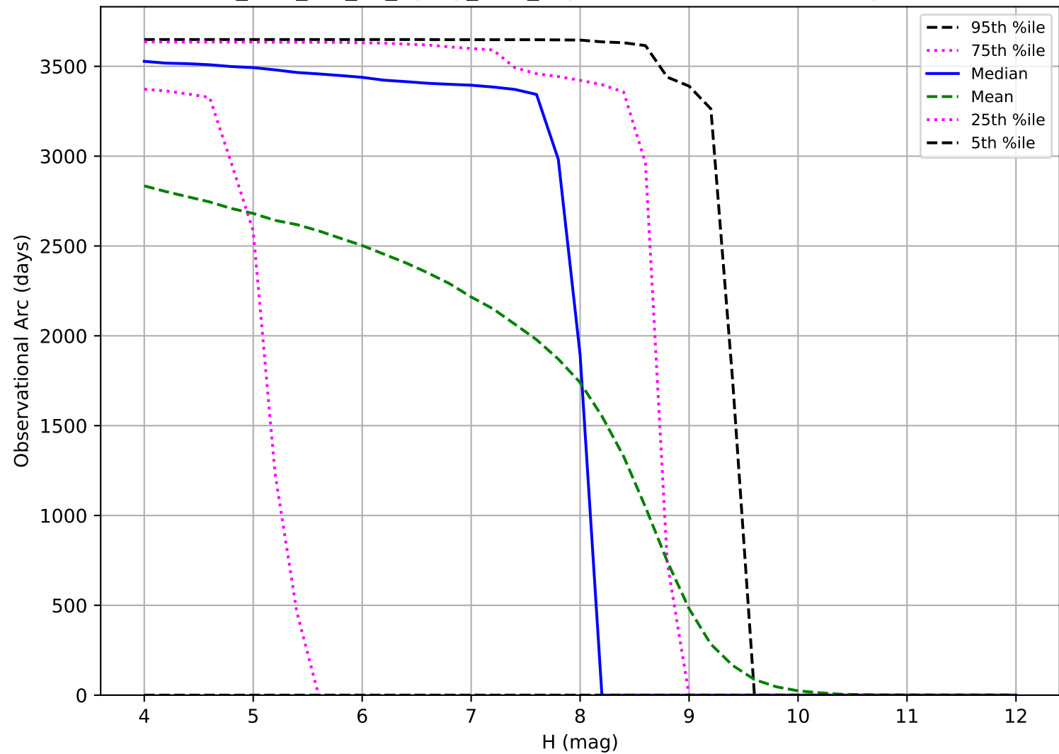
too_elab_r64_d2_ugrizy_v3.4_10yrs: Observational Arc Length TNO
