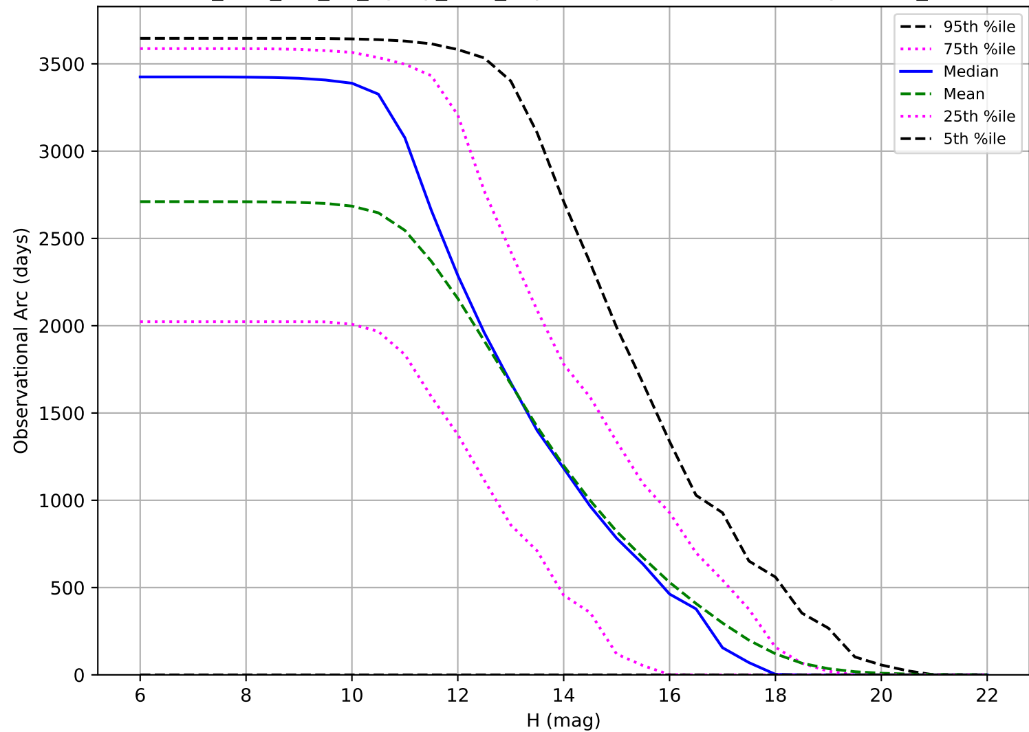
too_elab_r64_d2_ugrizy_v3.4_10yrs: Observational Arc Length OCC_r5
