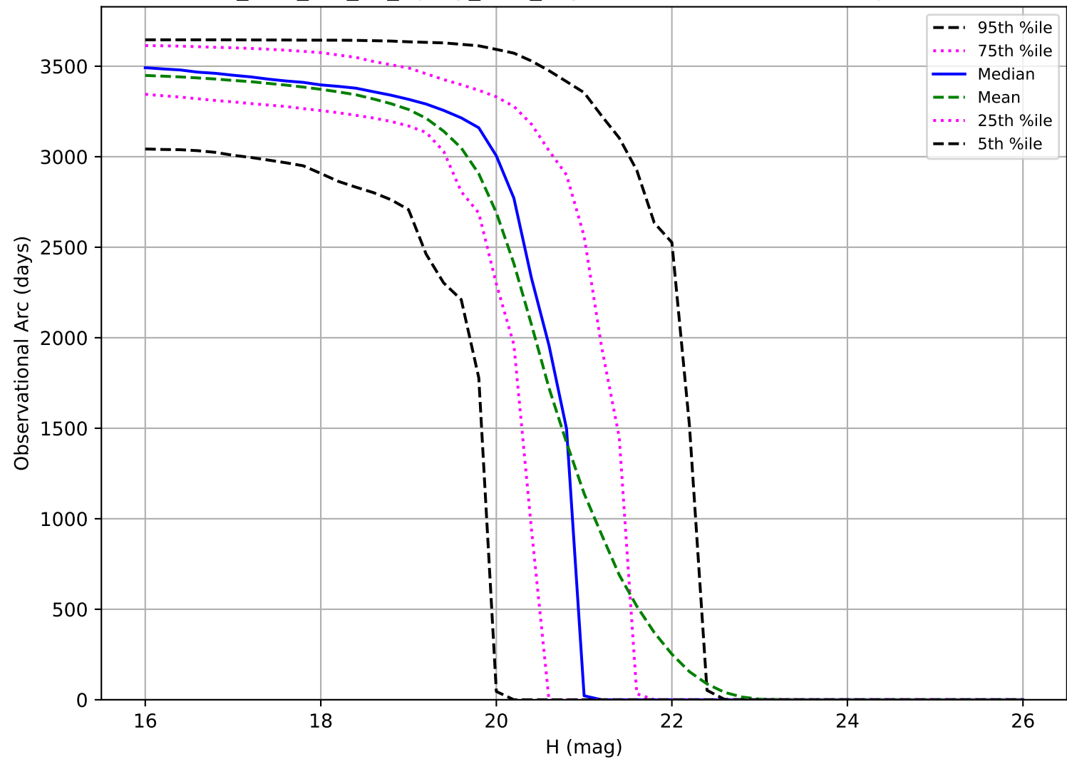
too_elab_r64_d2_ugrizy_v3.4_10yrs: Observational Arc Length MBA
