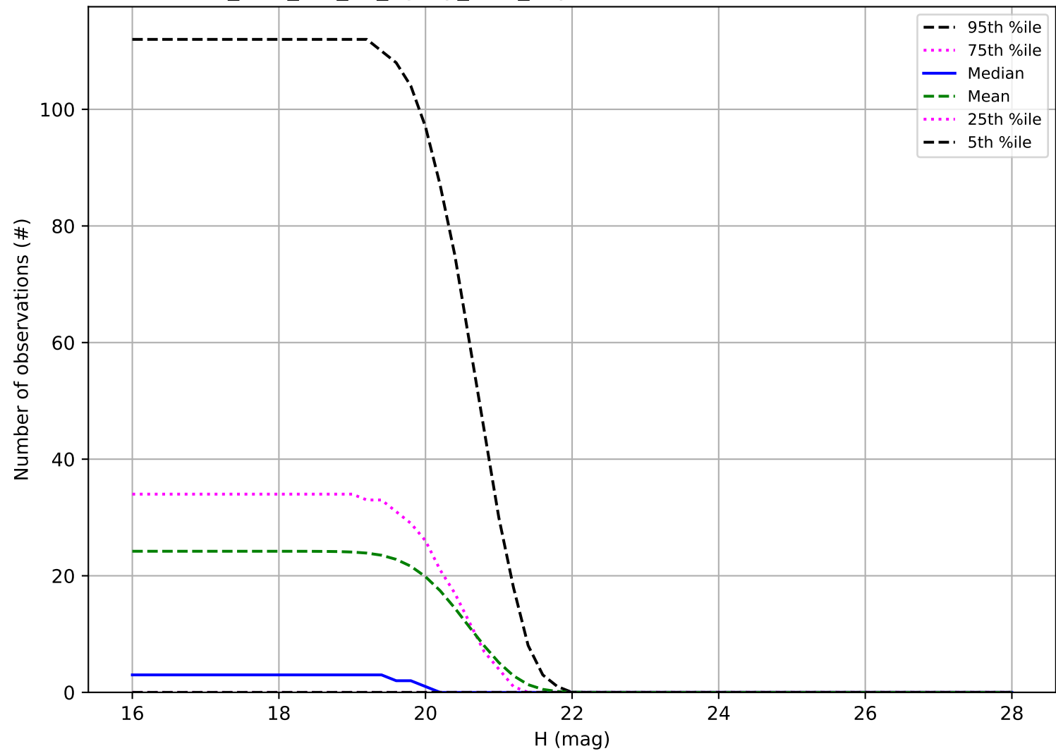
too_elab_r64_d2_ugrizy_v3.4_10yrs: Number of observations Vatira
