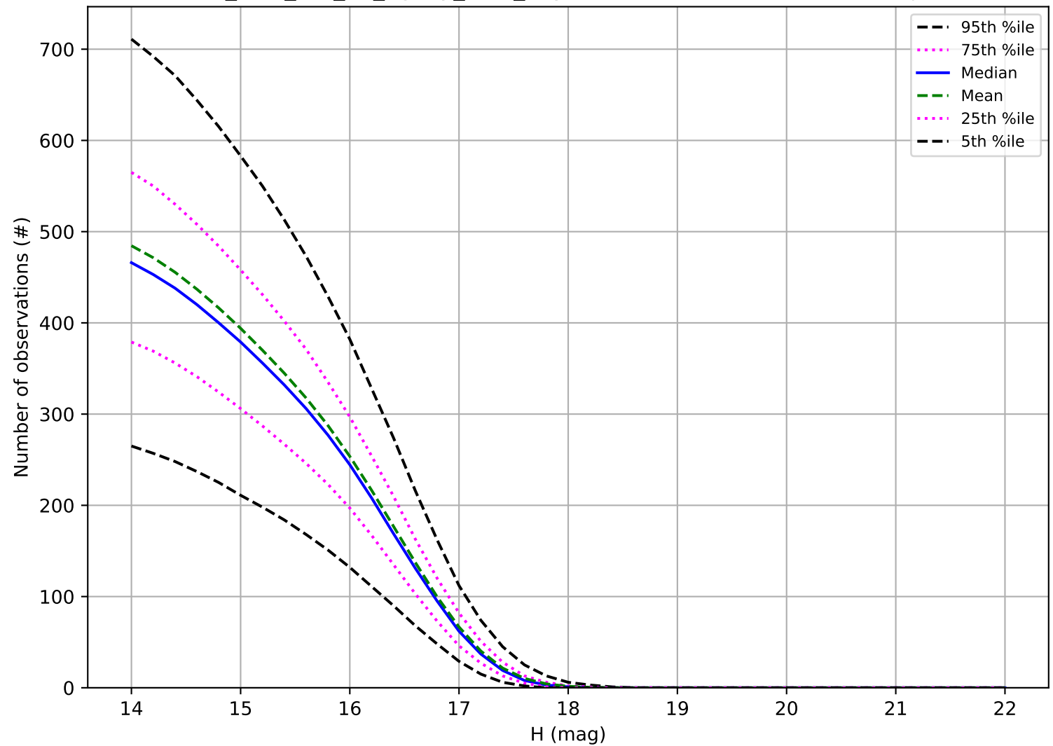
too_elab_r64_d2_ugrizy_v3.4_10yrs: Number of observations Trojan
