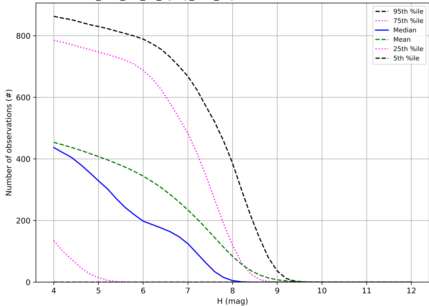
too_elab_r64_d2_ugrizy_v3.4_10yrs: Number of observations TNO
