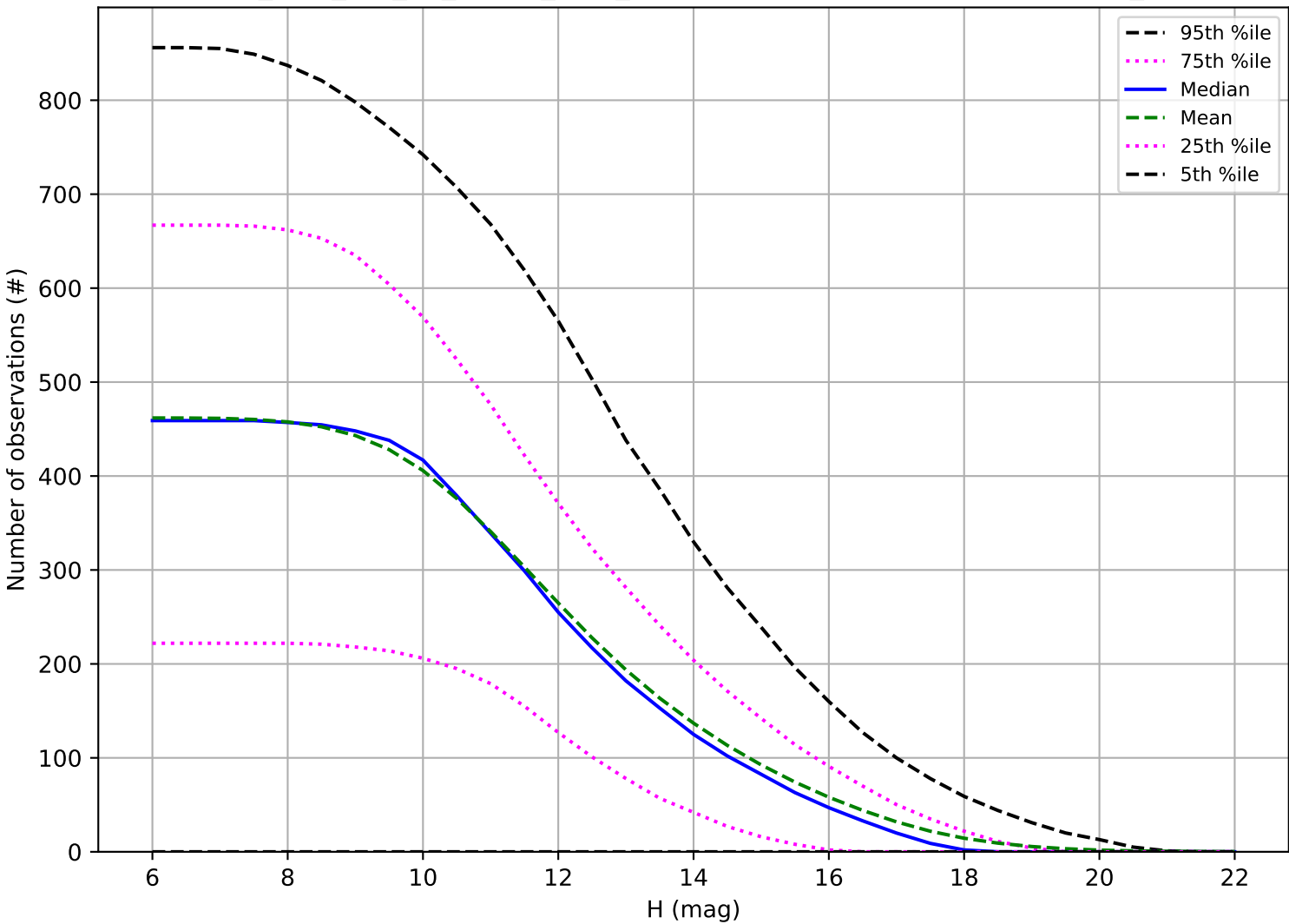
too_elab_r64_d2_ugrizy_v3.4_10yrs: Number of observations OCC_r5
