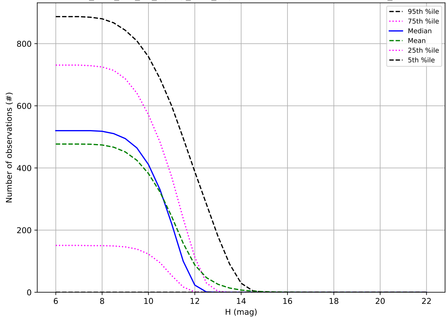
too_elab_r64_d2_ugrizy_v3.4_10yrs: Number of observations OCC_r20
